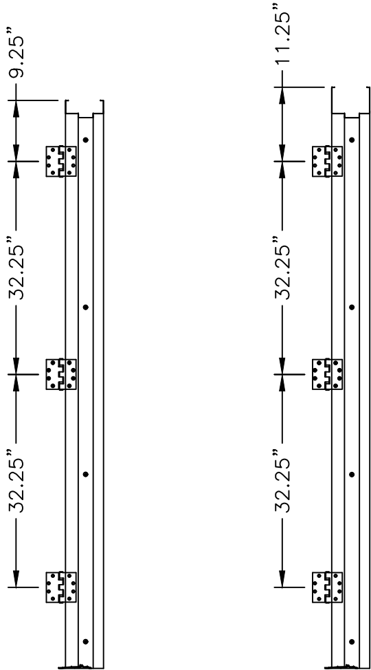
HINGE LOCATIONS HINGE LOCATIONS 2" HEAD 4" HEAD
