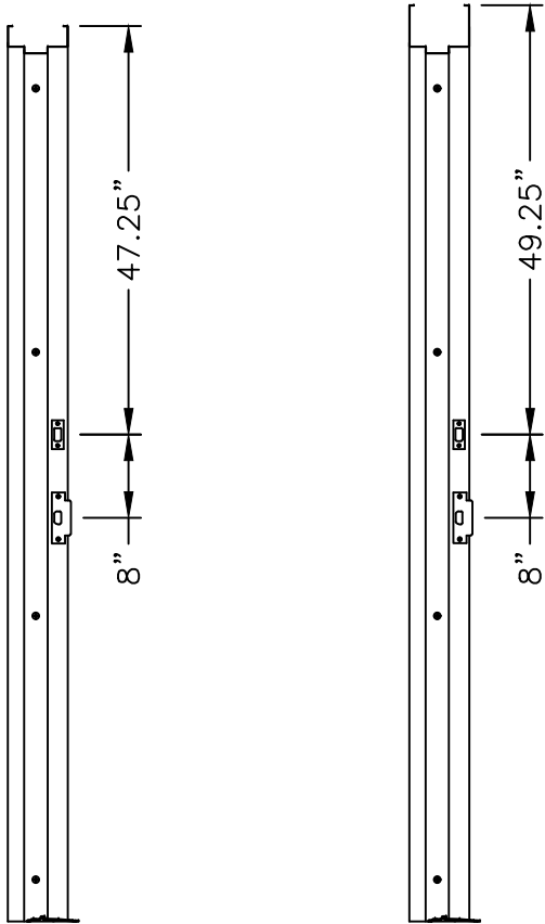
STRIKE PLATE STRIKE PLATE LOCATIONS 2" HEAD LOCATIONS 4" HEAD
