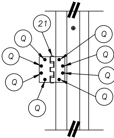
HINGE DETAIL
