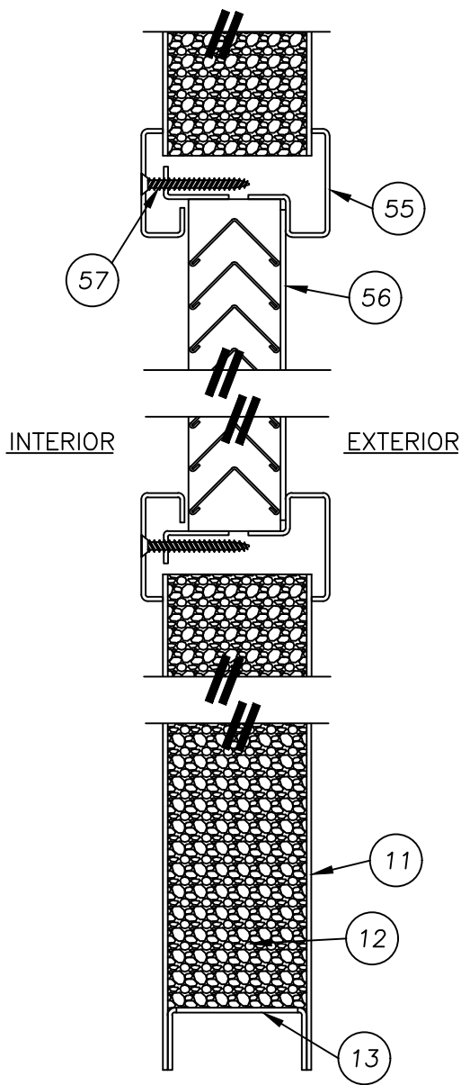
1/2 VERTICAL CROSS SECTION
