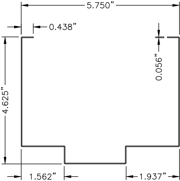
26 FRAME
