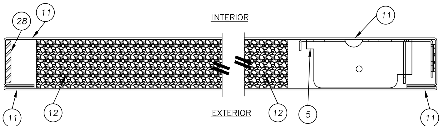
3/2 HORIZONTAL CROSS SECTION
