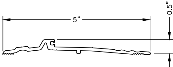
40 THRESHOLD
