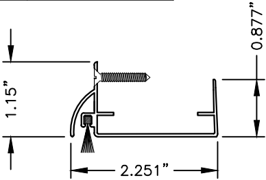
44 SWEEP
