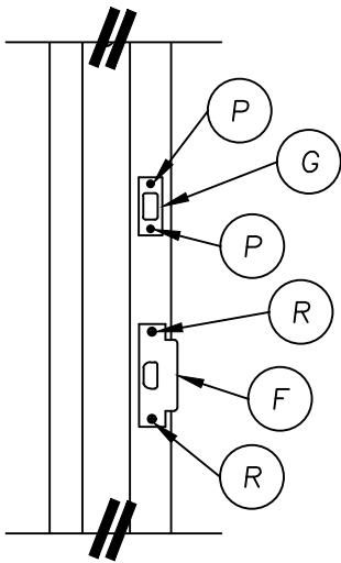
STRIKE PLATE DETAIL ANSI STRIKE & DEADBOLT
