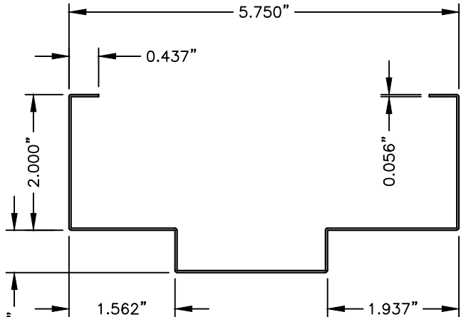
25 FRAME
