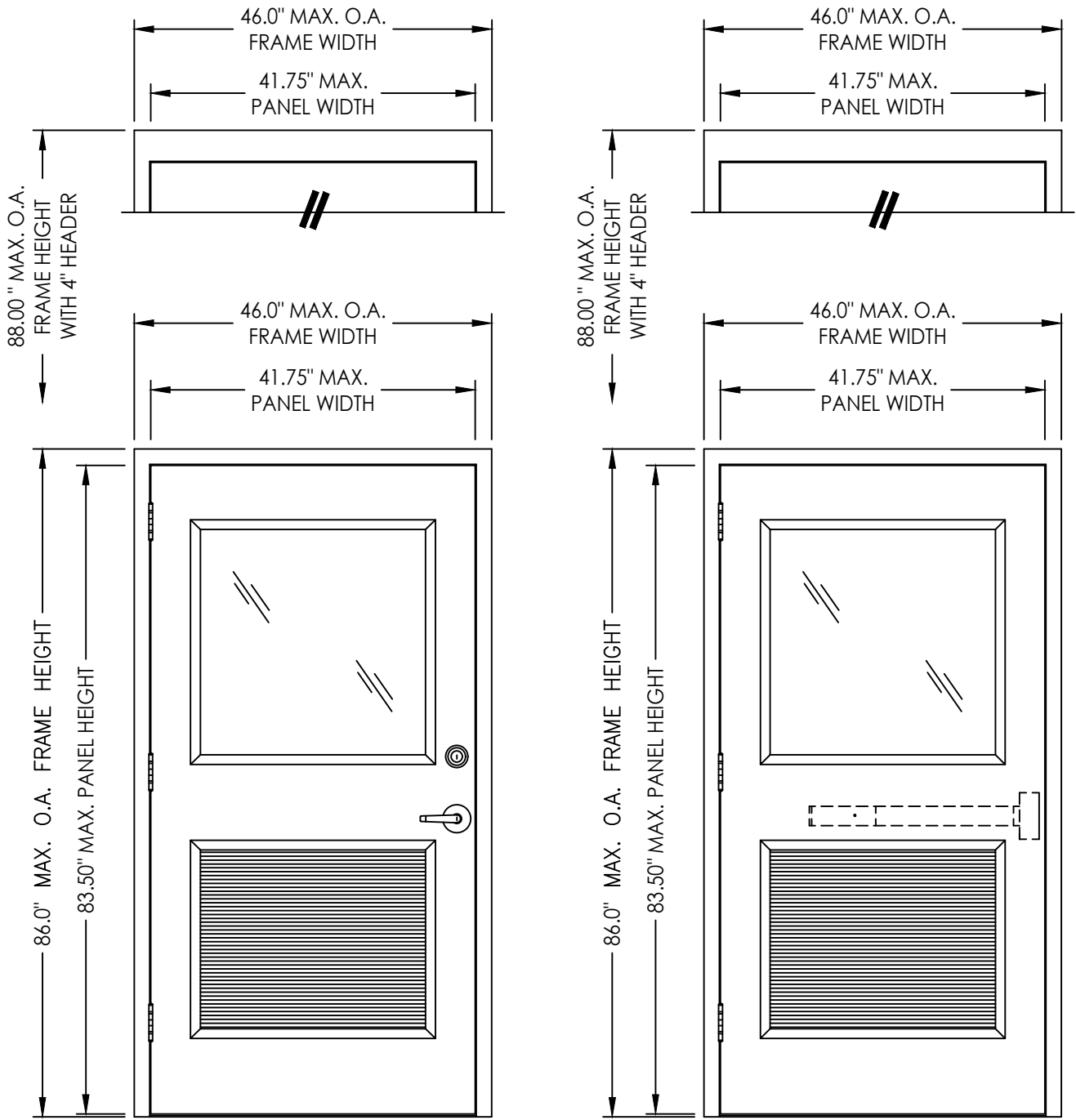
"N" DOOR
